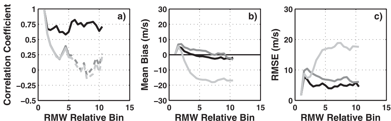
FIG. 6. Results of application of H10 (black), Emanuel in (4) (dark gray), and DeMaria in (5) (light gray) to 121 Atlantic SFMR surface wind profiles for (a) linear correlation, (b) bias ( \text{m s}^{-1} ), and (c) rmse ( \text{m s}^{-1} ). Significance at the 99% level is denoted by the solid part of the line in (a).
